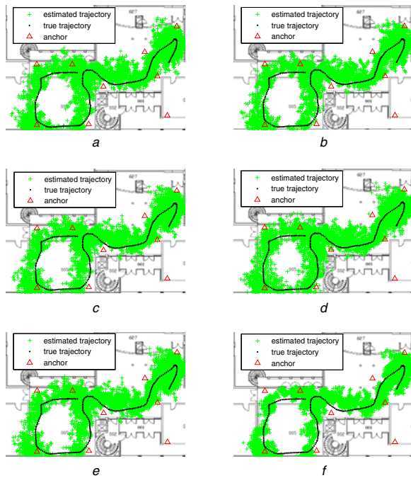
Fig. 1 Positioning behaviour of the smoothing methods on the building floor plan with classrooms and halls: the connected dots denote the ground truth of the mobile trajectory; the scatter plot '+' is the estimations; 'Δ' for the anchors
